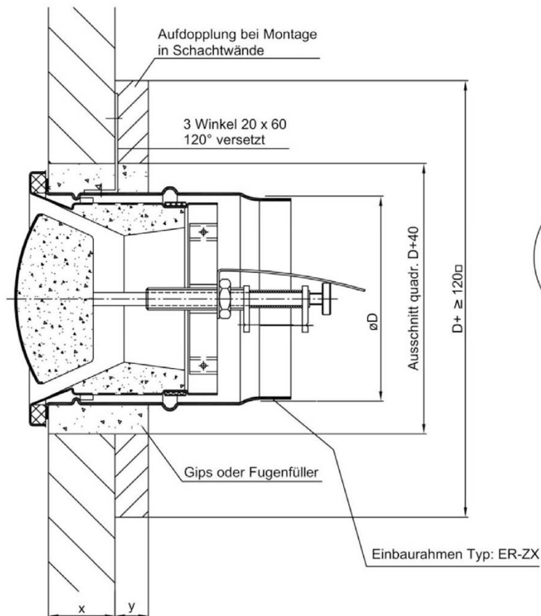
Detail A
